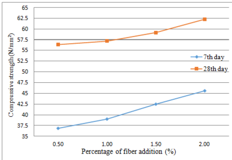
Figure 2. Impact of different steel fiber inclusion percentages on self-curing concrete's compressive strength
